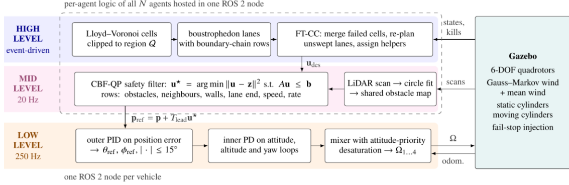
FIGURE 1. Three-layer architecture: per-agent layers, with the high and mid levels of all agents hosted in one ROS 2 node and one low-level controller per vehicle.
